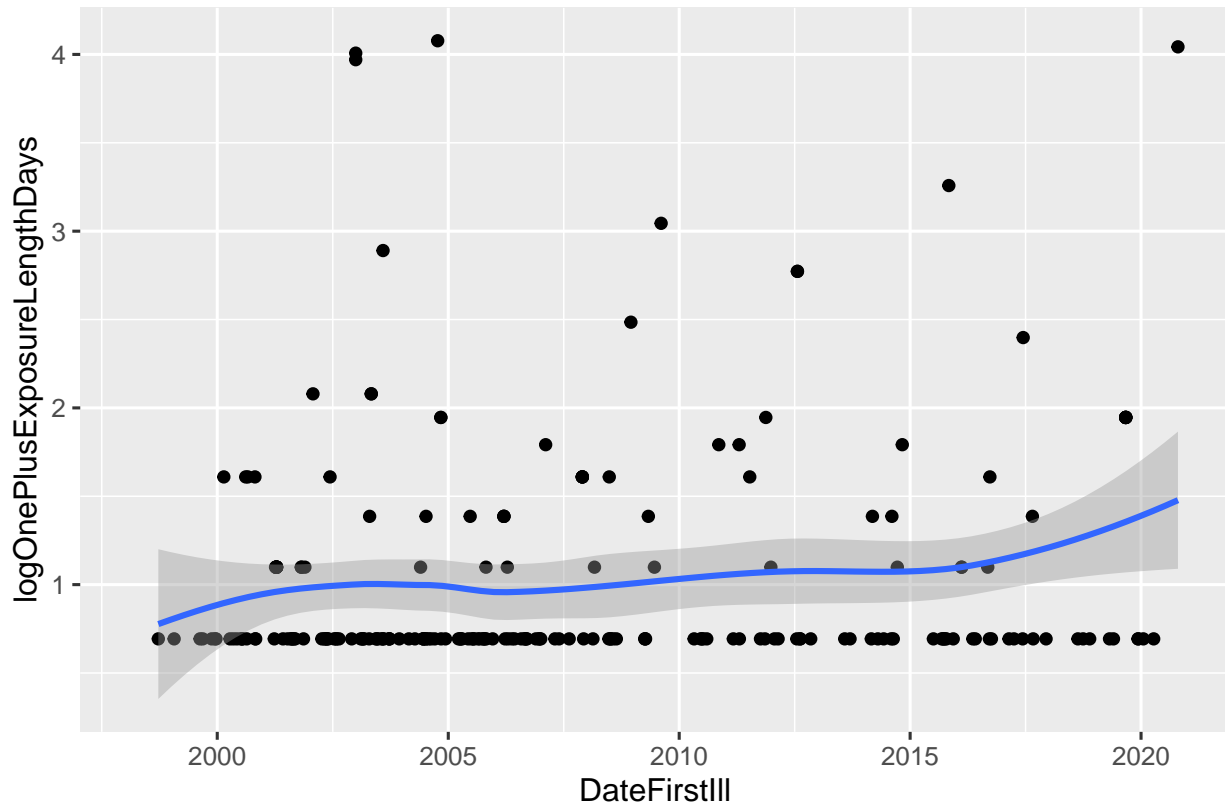
Figure D.2: Outbreak Length over Time. The LOESS curve ( \alpha = 0.5 , polynomial degree is 2) shows a prevailing flat trend. Though the ends suggest an upward trend, this is likely illusory; the lower end's confidence band comfortably includes the sample average, and the upper end is drawn up by the Minnesota COVID outlier outbreak.
