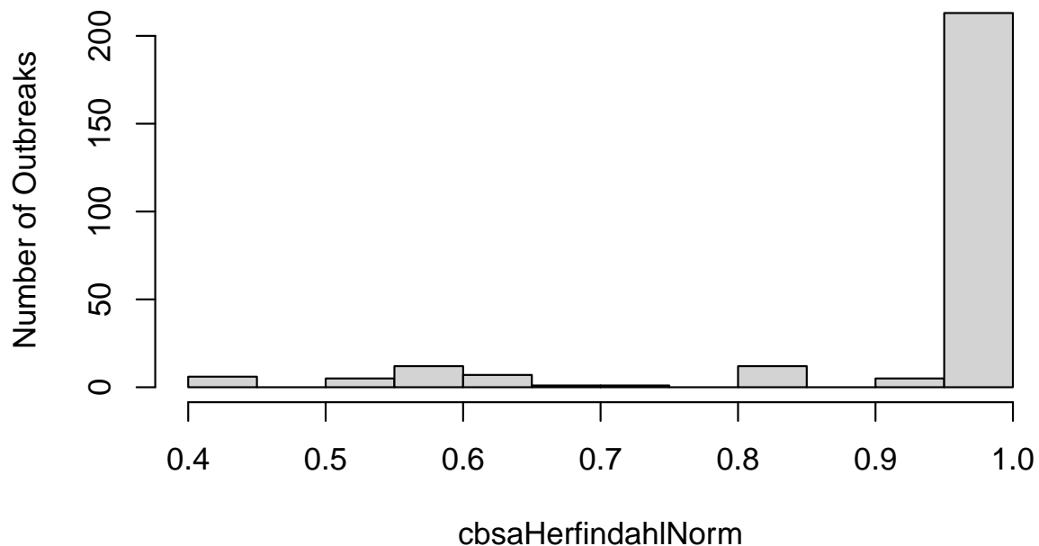
Figure D.1: Chemical Outbreaks by Metro Concentration.
