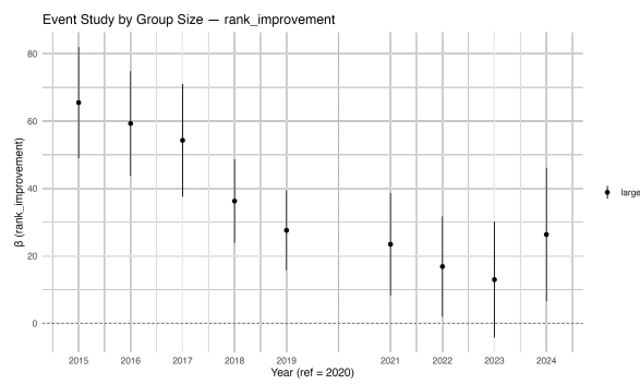
Figure 28: Rank-improvement coefficients by group-size bins (95% CIs).
