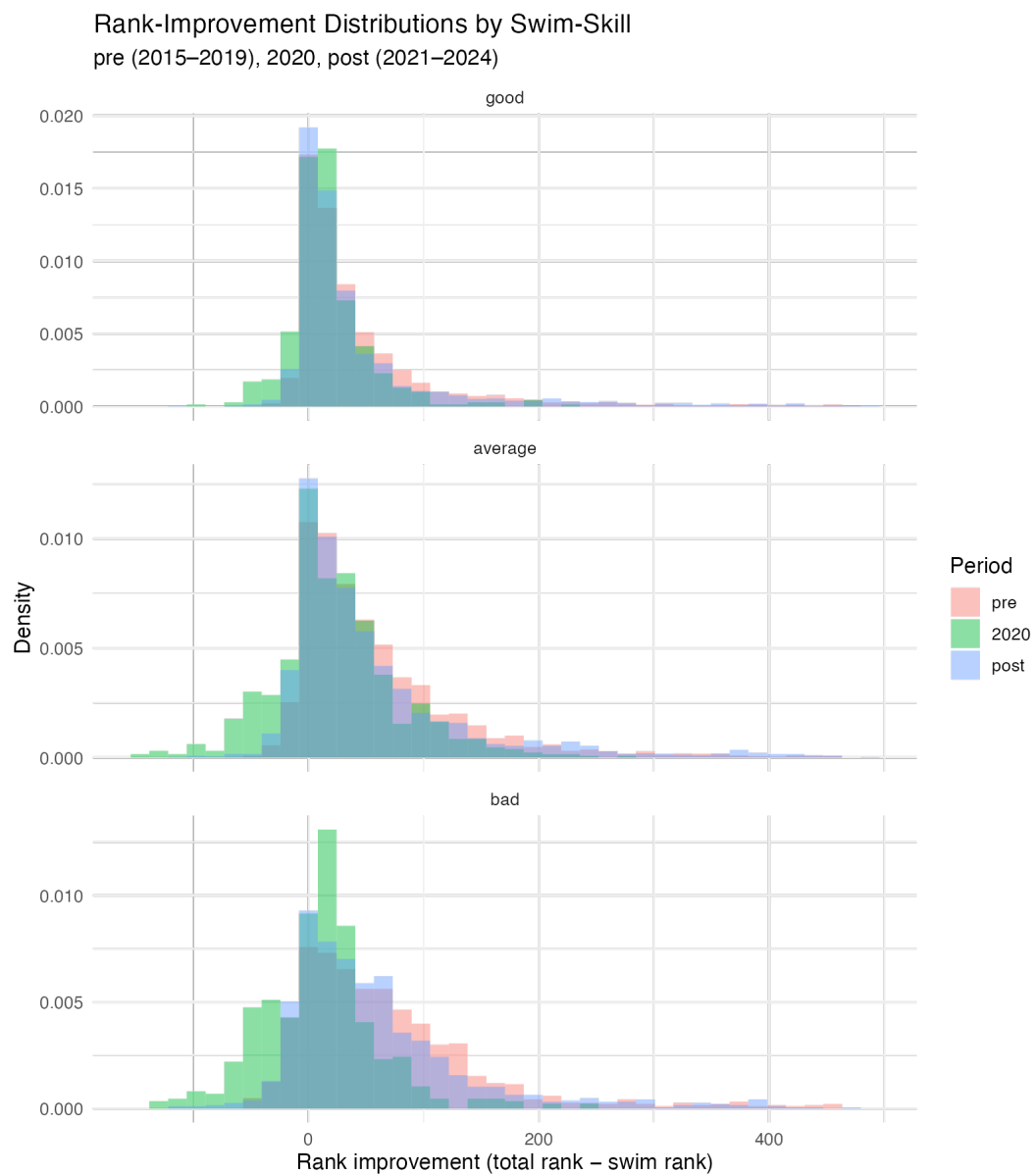
Figure 7: Distributions of rank improvements by swim skill and period (pre, 2020, post). Conclusion: \text{Pre} \succeq \text{Post} \succeq 2020
