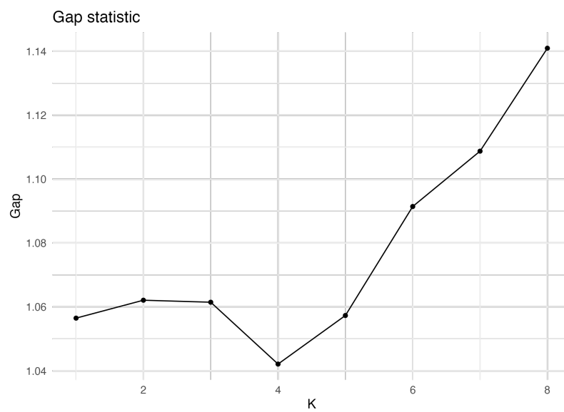
Figure 42: Gap statistic \text{Gap}(k) with one-SE rule.
