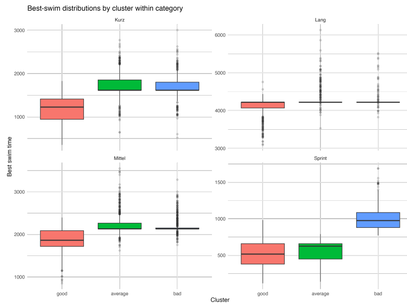
Figure 45: Swim times by cluster and event category (IQR boxes, 1.5 \times \text{IQR} whiskers). Median times follow good < average < bad .
