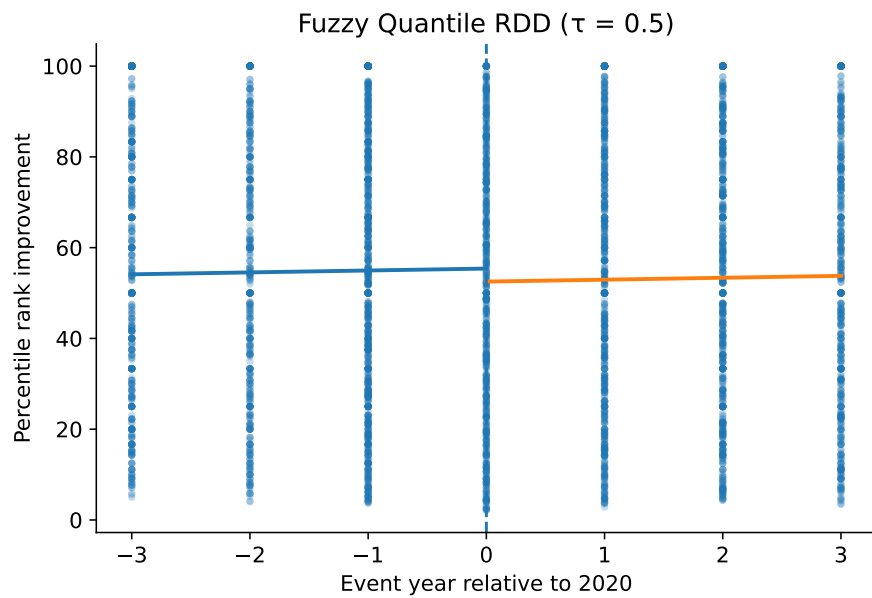
Figure 15: Fuzzy Quantile Regression Discontinuity at the Median
