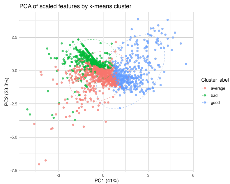
Figure 43: PCA projection of athletes with k = 3 clusters and 95% ellipses.
