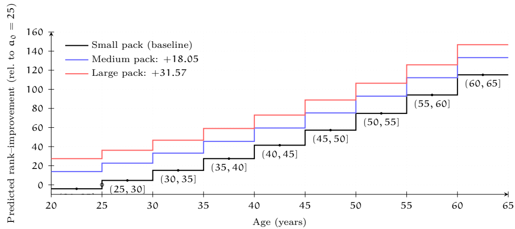
Figure 32: Age heterogeneity (step function) including all pack-size groups . Lines show model-implied predictions by age bin using \widehat{\Delta RI}(a) = 0.0351(a^2 - 25^2) , with vertical shifts of +18.05 (medium) and +31.57 (large) relative to the small-group as baseline group.
