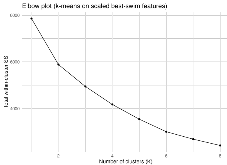
Figure 40: Elbow plot: within-cluster dispersion W_k as a function of k .
