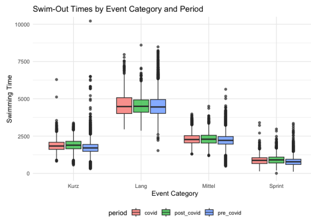
Figure 4: Swim-out times by event category and period (original sample). Boxes show the interquartile range; whiskers extend to 1.5 \times \text{IQR} .
