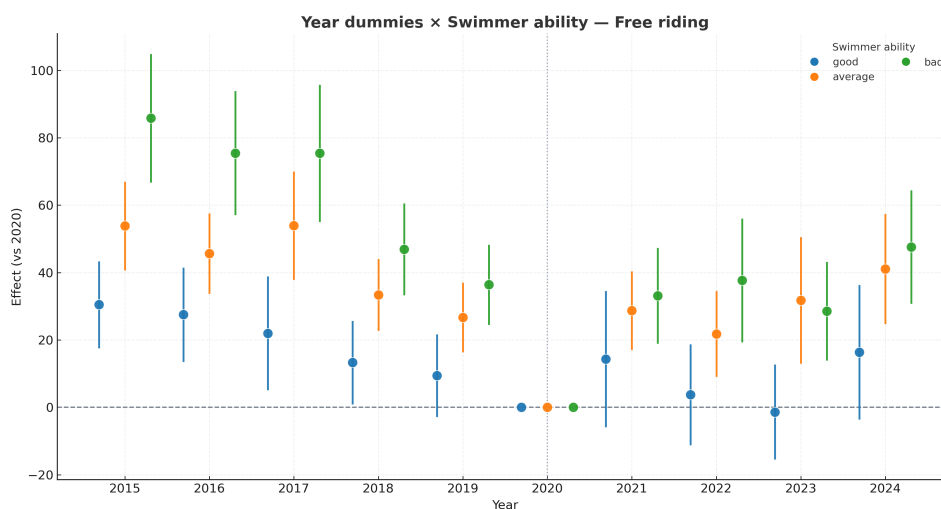
Figure 25: Year×swimmer ability event–study for free–riding (good/average/bad). 95% CIs; ref = 2020.
