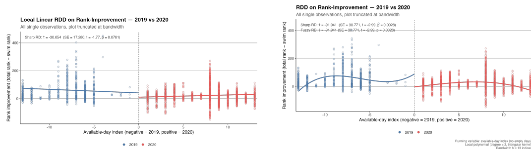
(b) Local linear fit ( p = 1 ) with triangular kernel weights. Blue points: 2019 ( x < 0 ), red points: 2020 ( x > 0 ).
