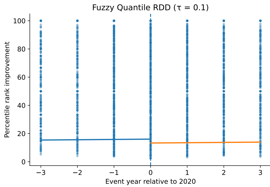
Figure 14: Fuzzy Quantile Regression Discontinuity at the 10th Percentile
