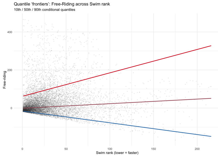
Figure 36: Estimated conditional quantile frontiers Q_{\tau}(\text{FR} \mid r) at \tau \in \{0.10, 0.50, 0.90\} . The \tau = 0.90 curve serves as a proxy for the frontier \text{FR}^*(r) ; higher \tau values tighten the approximation, subject to sampling variability.
