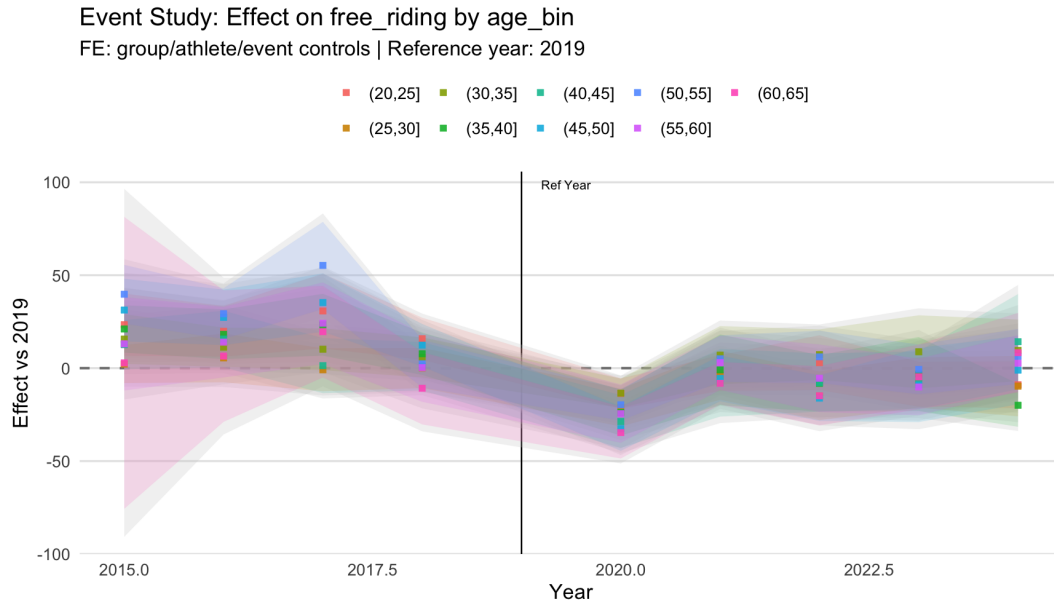
Figure 31: Year FEs by Age bin (20–25, . . . , 60–65), baseline=2019.
