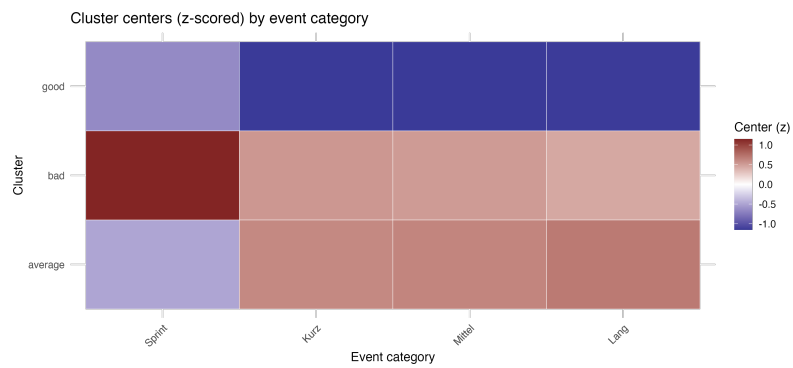
Figure 44: Cluster centroids across event categories (z-scored).
