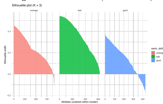
Figure 47: Silhouette widths by athlete for k = 3 .
