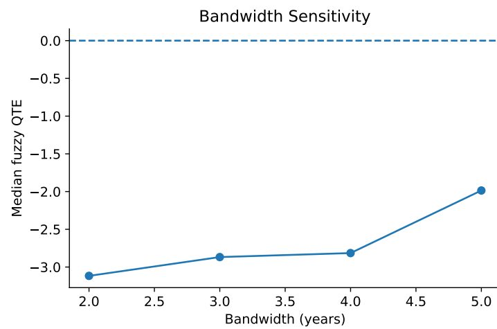
Figure 17: Bandwidth Sensitivity of Median Fuzzy QTE
