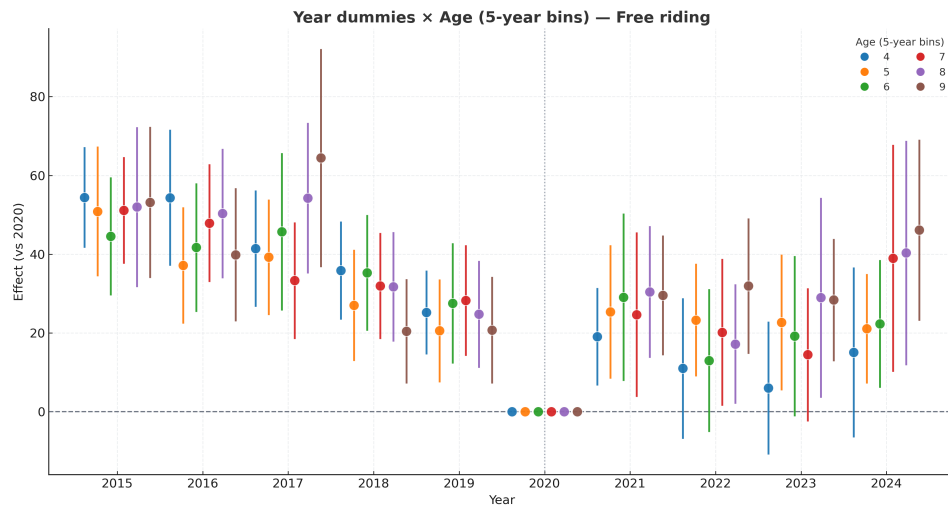
Figure 23: Year×age-bin event-study for free-riding. Bins ordered by lower bound; candlesticks show 95% CIs; ref = 2020.
