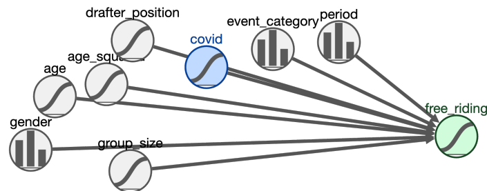
Figure 48: Directed acyclic graph (DAG) used for identification.
