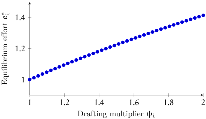
Figure 2: Equilibrium Effort as a Function of Drafting
