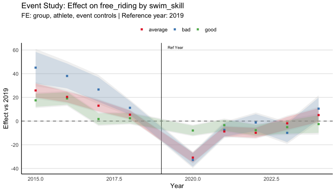
Figure 30: Year FEs by Swim Ability (Good/Bad/Average), baseline=2019.
