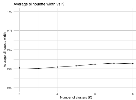
Figure 41: Average silhouette \bar{s}(k) .
