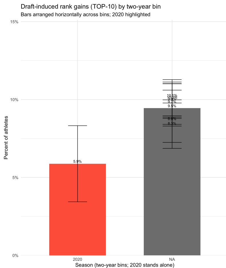
Figure 10: Draft-induced rank improvements among TOP-10 athletes by two-year bins; the COVID season (2020) is shown separately.
