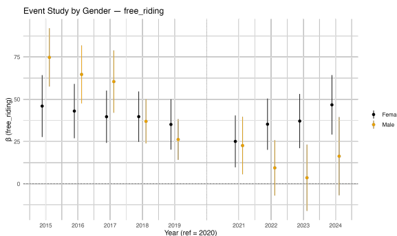
Figure 20: Year×gender coefficients for free–riding (points = estimates, bars = 95% CIs).
