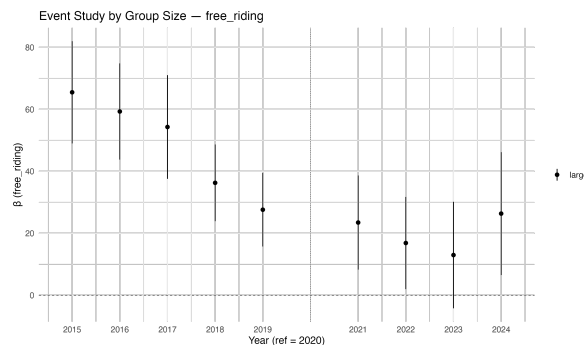
Figure 27: Free–riding coefficients by group–size bins (95% CIs).
