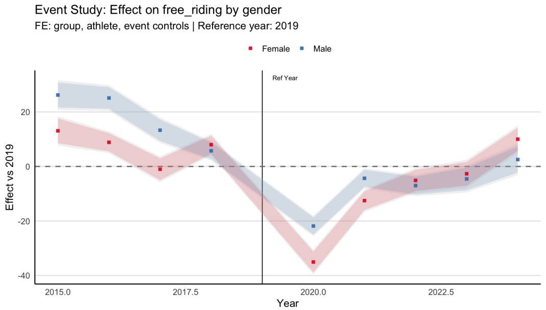
Figure 29: Year FEs on Free Riding by Gender (Male vs. Female), baseline=2019
