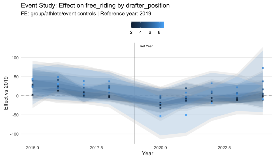
Figure 33: Year FEs by Drafter Position (1–8), baseline=2019.
