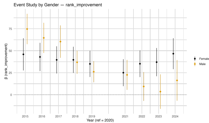
Figure 21: Year×gender coefficients for rank-improvement (95% CIs).
