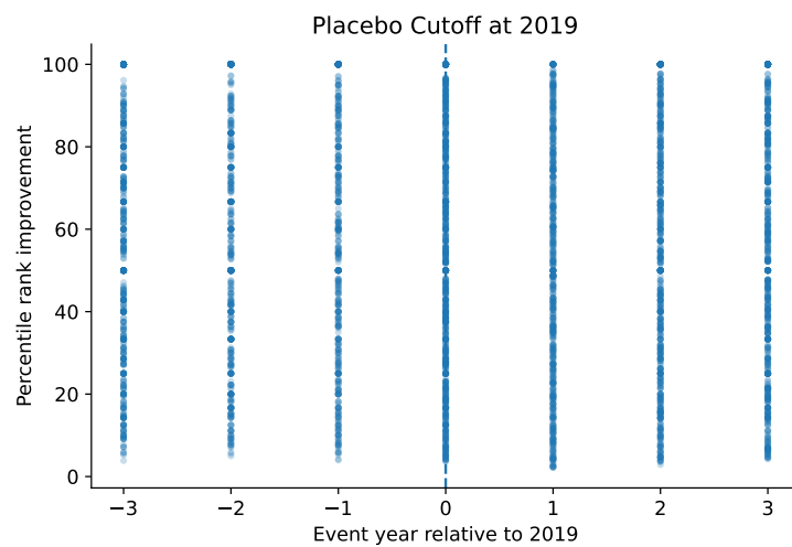
Figure 19: Placebo Cutoff at 2019
