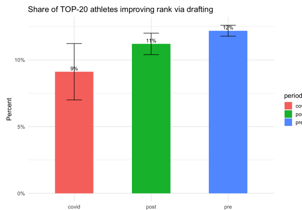
Figure 12: Share of TOP-20 athletes improving rank via drafting by period.
